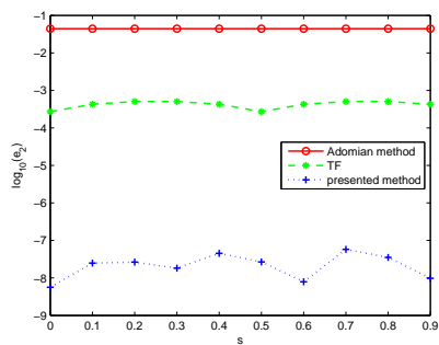
Figure 8. Comparison e_2 of the Adomian method in [6] and TF method in [5] with presented method for example 6.2
